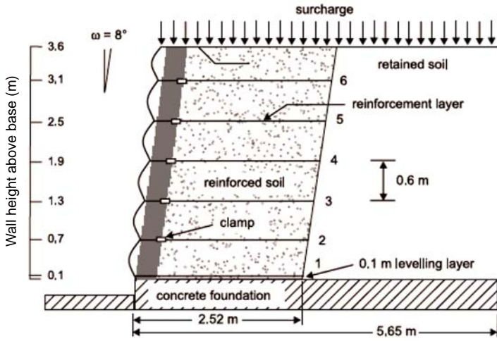
Fig. 4 Cross-section of the GRS test wall (Bathurst et al. 2006)
