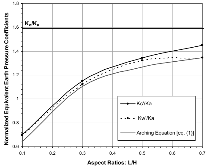
Fig. 8 Normalized equivalent earth pressure coefficients for at-rest case
